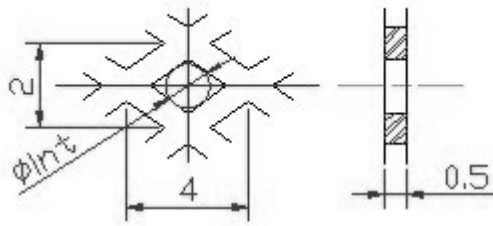
Filter 1/2" -> 2" \phi_{int} max = 1mm.
